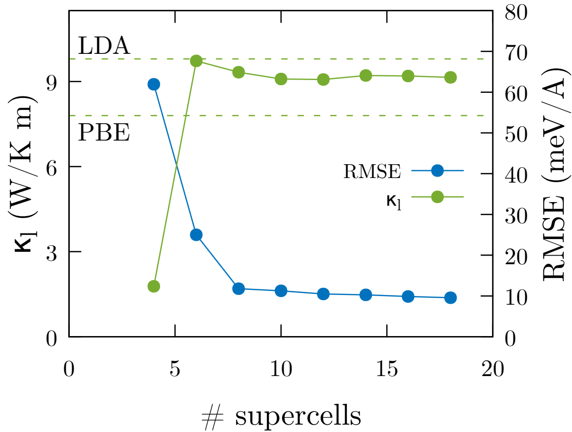
Figure 1. Lattice thermal conductivity of \text{CoSb}_3 as a function of the number of supercells used in the machine learning model (green circles) and the root mean square error of the forces for each model (blue circles). Dashed green lines represent the lattice thermal conductivity calculated with LDA and PBE functionals using the traditional approach in Ref [5]. Lattice parameters for \text{CoSb}_3 , LDA: 8.92 Å, PBE: 9.11 Å, PBE+D3: 9.03 Å, experimental: 9.04 Å. Experimental values reported for \text{CoSb}_3 lattice thermal conductivity are around 10 W/(m K).
