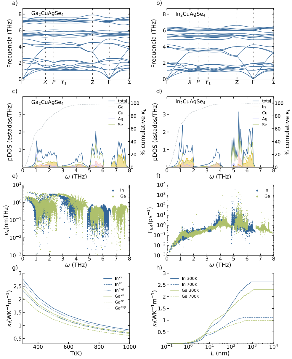
Figure 2. Dispersion curves (a-b), phonon density of states, pDOS, (c-d), group velocities (e), scattering rates (f) and lattice thermal conductivity (g-h) for \text{Ga}_2\text{CuAgSe}_4 and \text{In}_2\text{CuAgSe}_4 quaternary chalcogenides.
