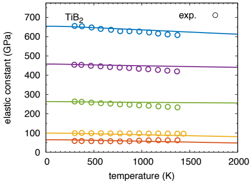
Comparison of calculated (lines) and experimental (circles) elastic constants for \text{TiB}_2 at different temperatures.
