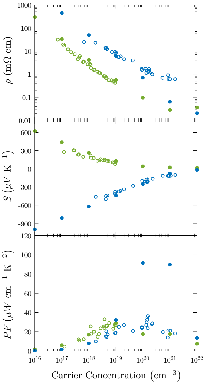
Fig 1. a) Resistivity, \rho , b) Seebeck coefficient, S , and c) power factor, PF for \text{CoSb}_3 . Empty and filled circles represent experimental data for monocrystalline samples and calculated values with AMSET, respectively. Colors: green = p-type, blue = n-type semiconductor.
