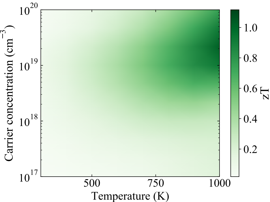
Fig 2. Figure of merit, zT , for p-type \text{CoSb}_3
