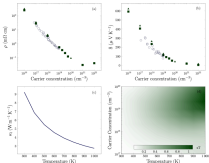
Fig. 4. (a) Resistivity, \rho , and (b) Seebeck coefficient, S , of \text{CoSb}_3 at 300 K. Blue empty circles represent experimental data and the Green filled triangles and squares represent calculated values with two different DFT functionals. (c) Calculated lattice thermal conductivity between 300 K and 1000 K. (d) zT for p-type \text{CoSb}_3 .
