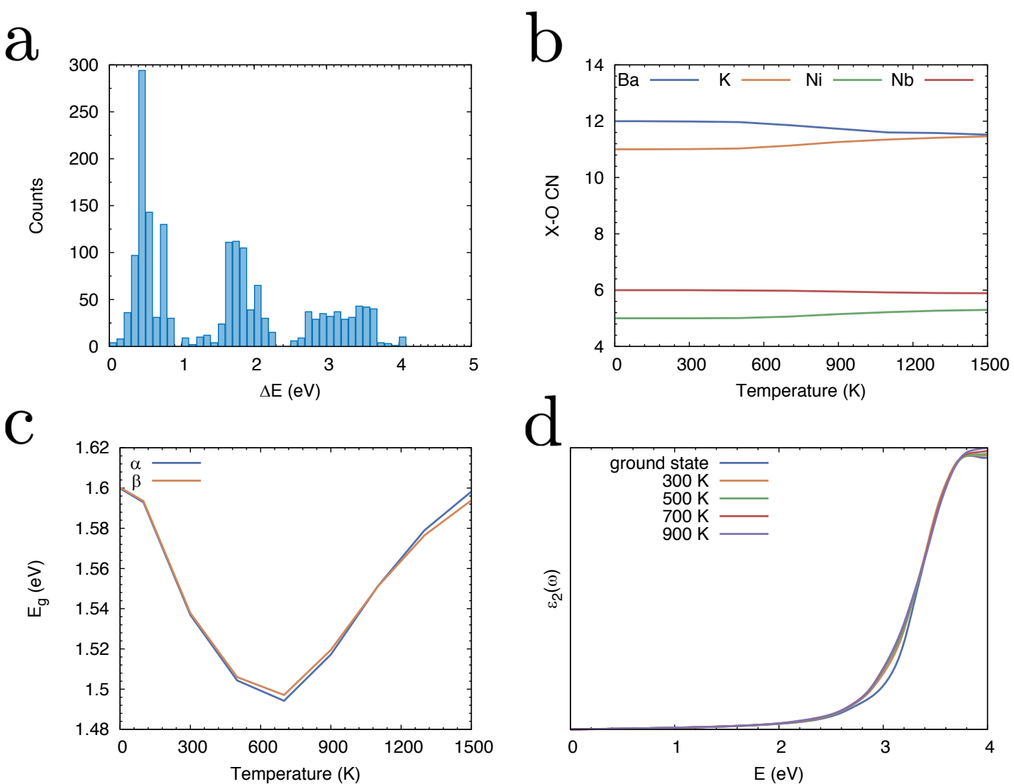
Figure 1. a ) Histogram with relative energies, \Delta E , for all the structures explored for the 0.5\{\text{KNbO}_3\}-0.5\{\text{Ba}(\text{Ni}_{0.5}\text{Nb}_{0.5})\text{O}_{3-\delta}\} system; b ) Coordination number, CN, for each cation, X, at different temperatures; c ) PBE+U band gap, E_g , for the majority, \alpha , and minority, \beta , spin at different temperatures; d ) Simulated spectra using the imaginary part of the dielectric function at different temperatures.
