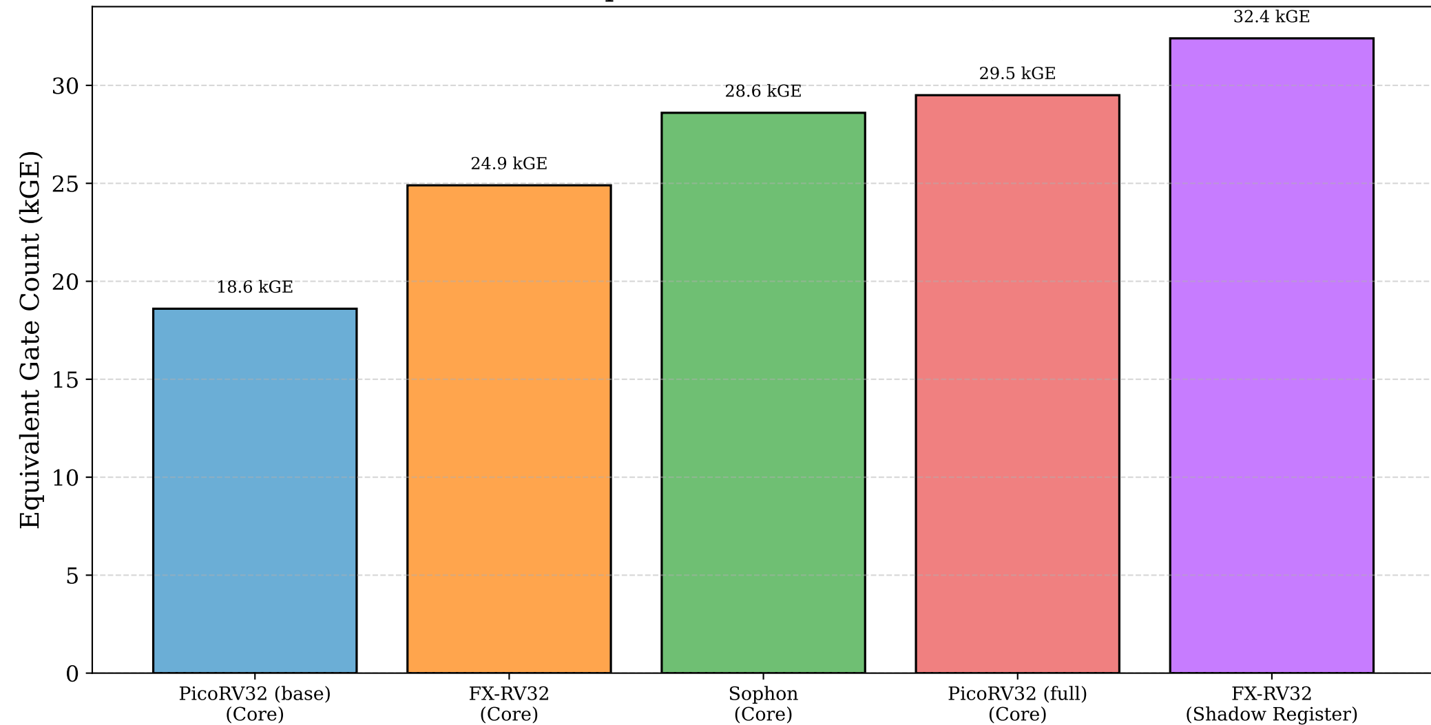
Area Comparison of RISC-V Cores (kGE)
