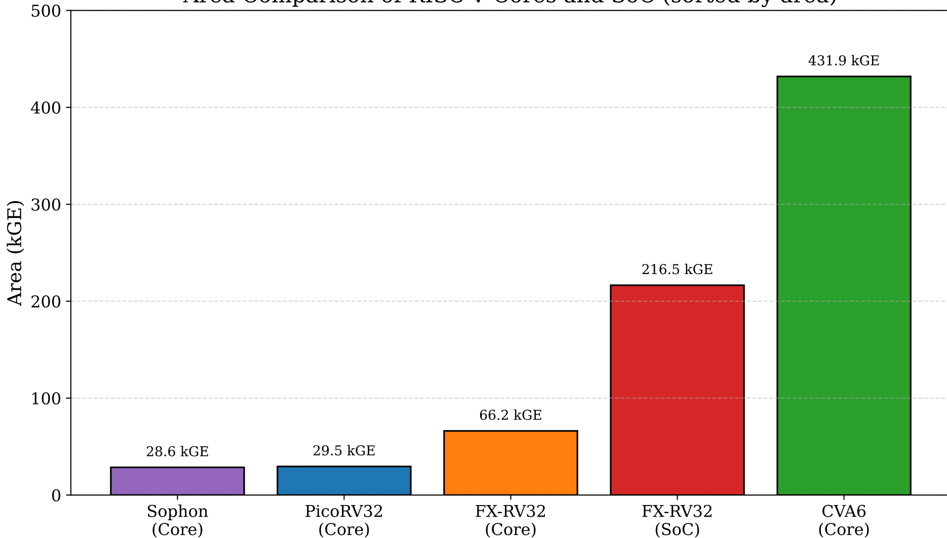
Area Comparison of RISC-V Cores and SoC (sorted by area)
