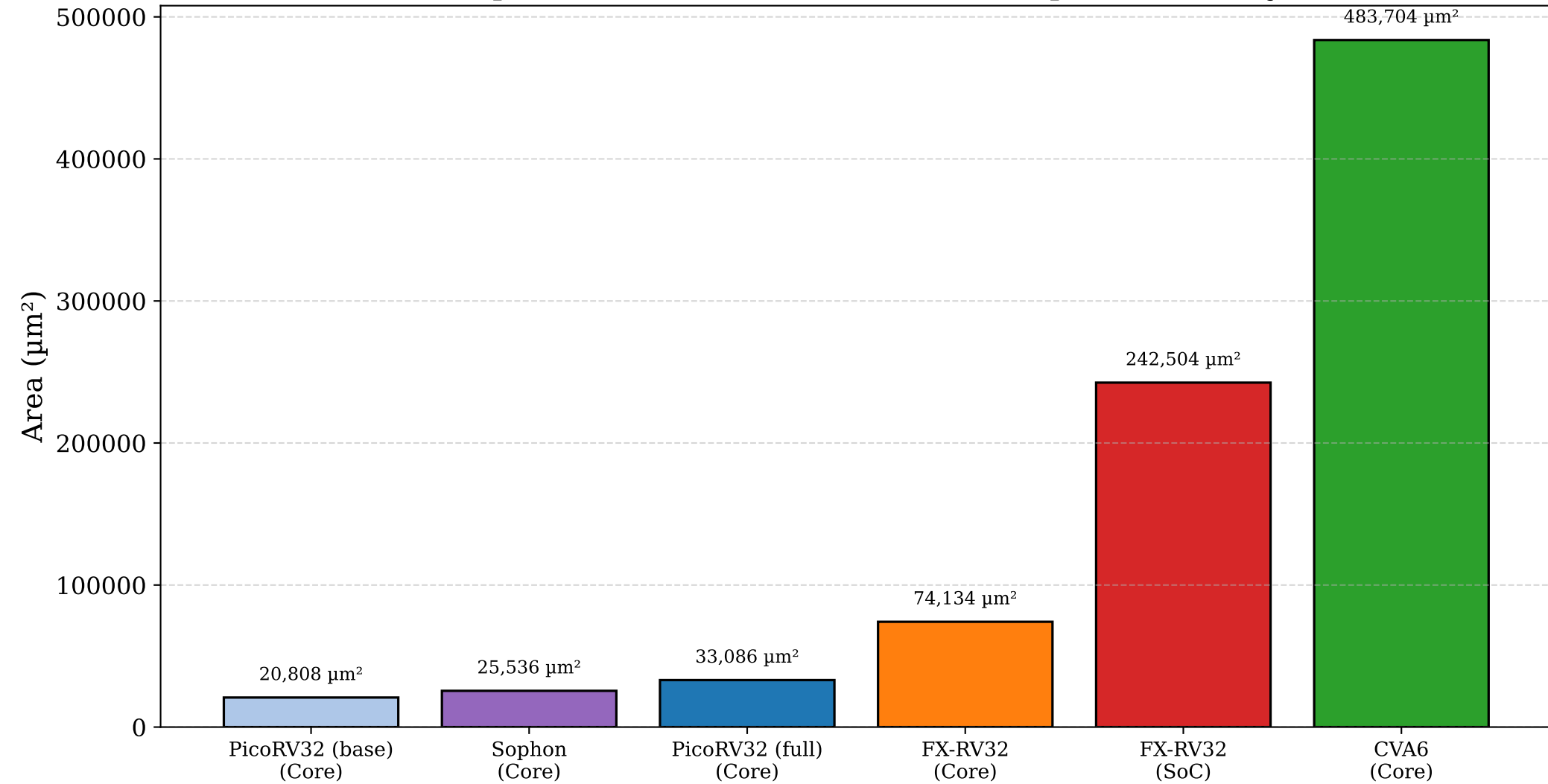
Area Comparison of RISC-V Cores and SoC ( \mu\text{m}^2 , sorted by area)
