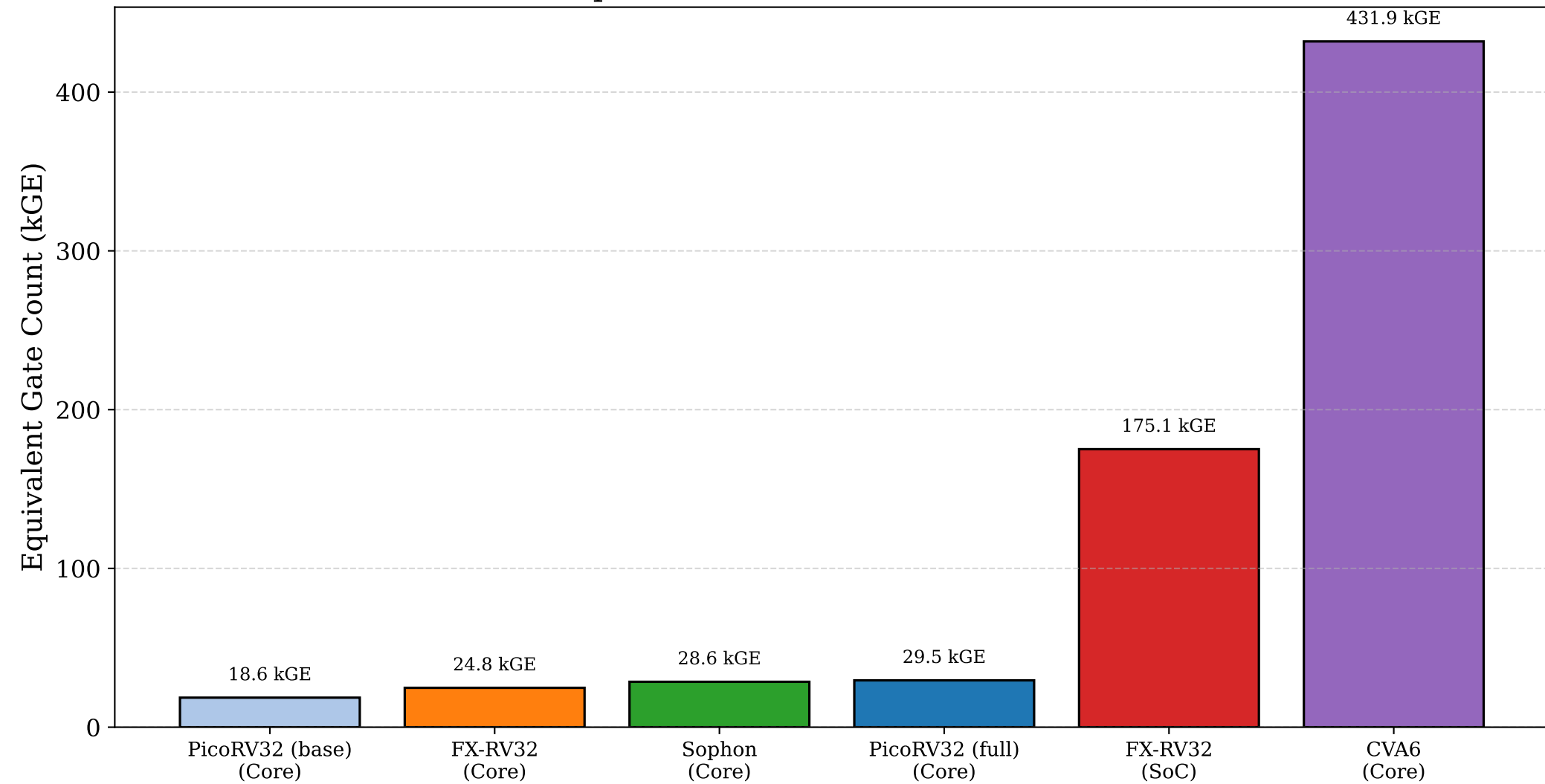
Area Comparison of RISC-V Cores and SoC (kGE)
