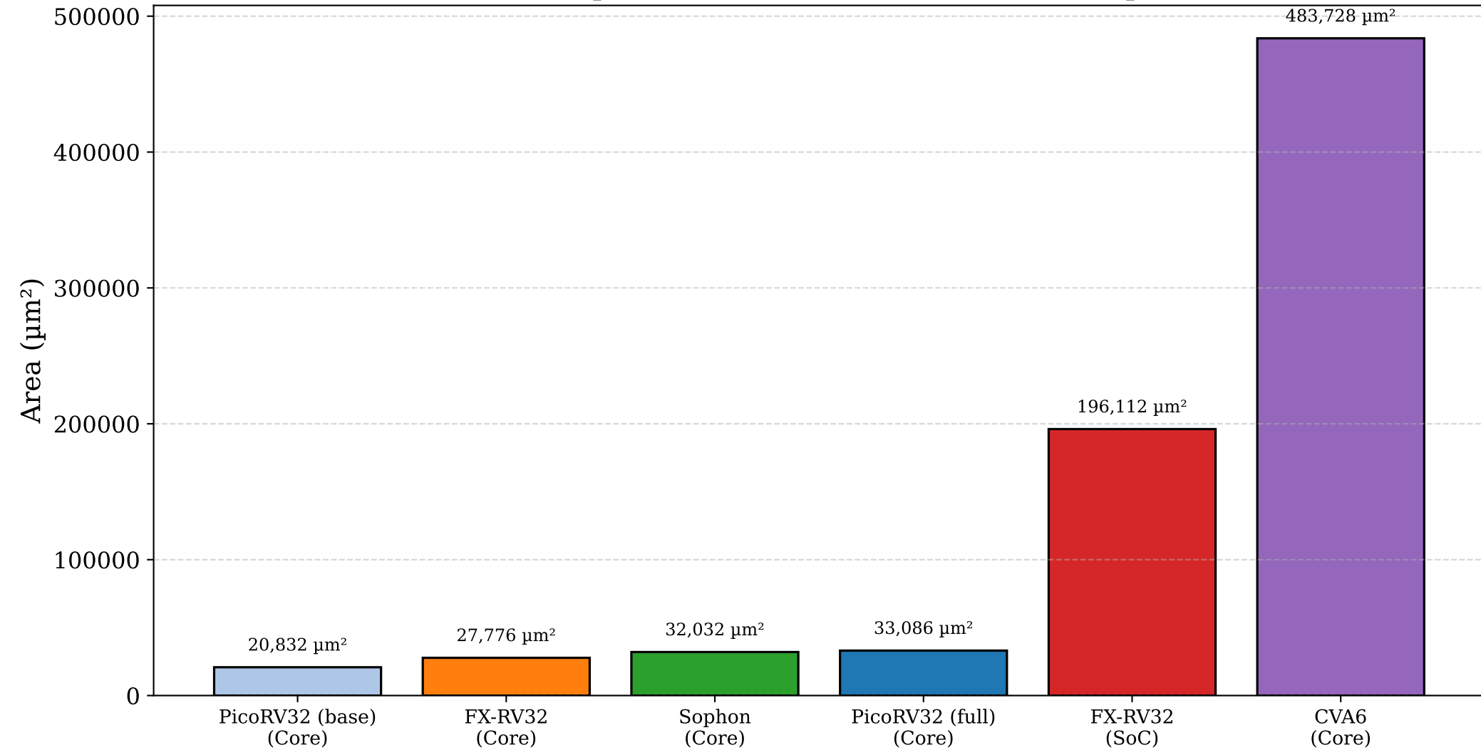
Area Comparison of RISC-V Cores and SoC ( \mu\text{m}^2 )
