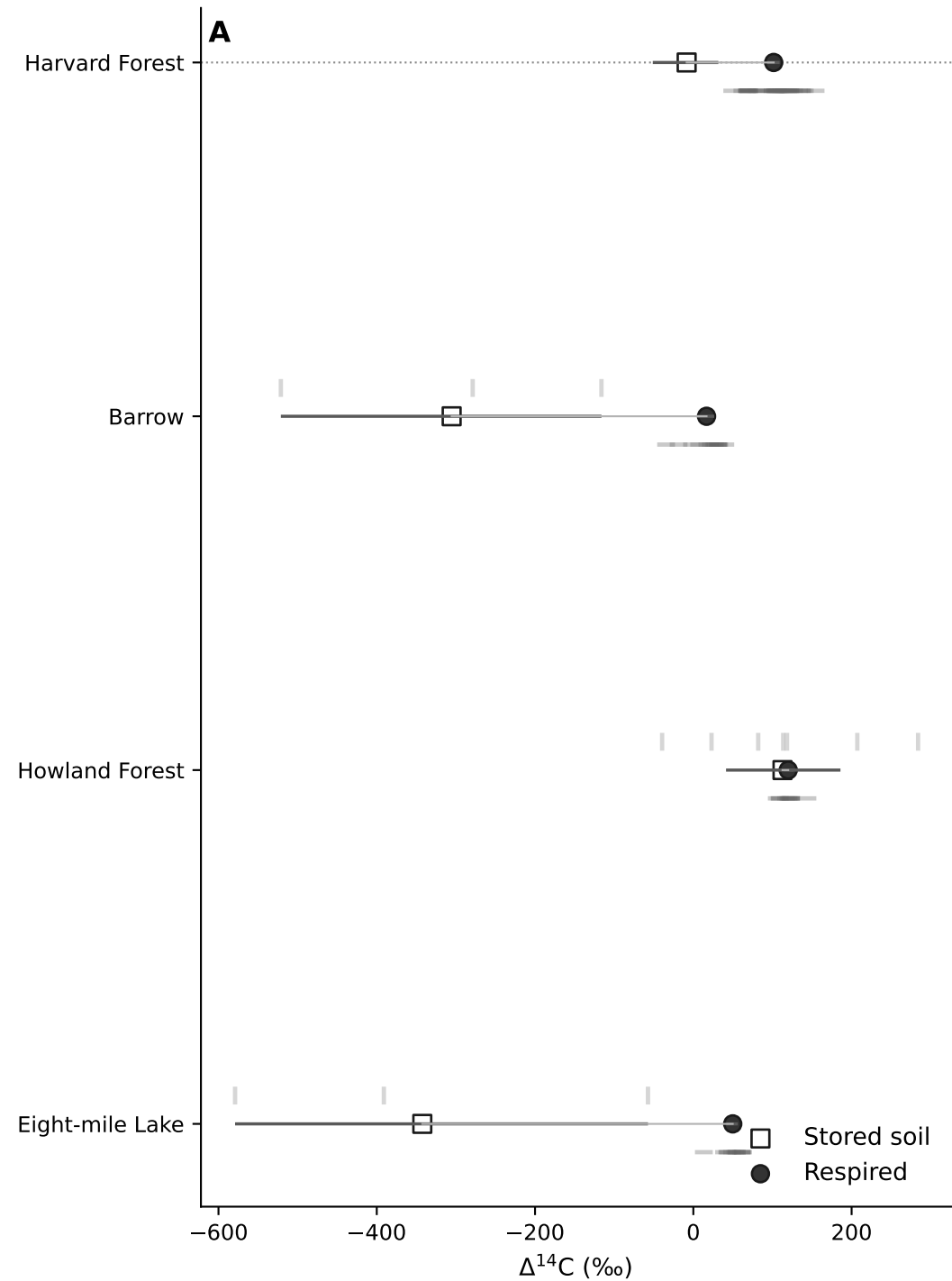
Stored-Soil and Respired \Delta^{14}\text{C} by Ecosystem
