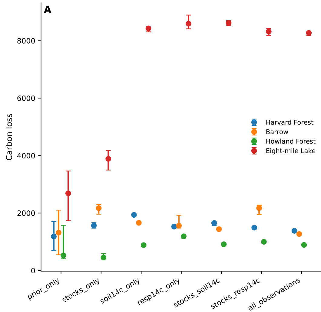
Total Carbon Loss at 100 Years
