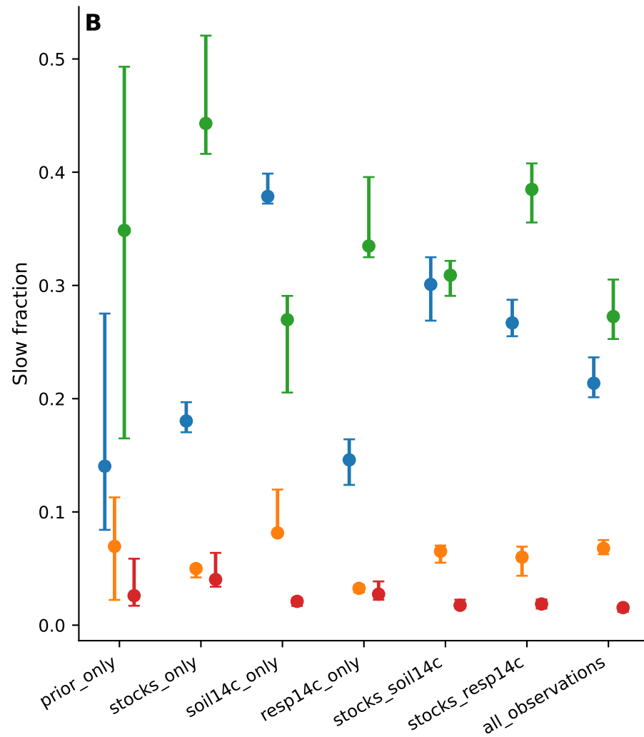
Slow Fraction of Excess Respiration at 100 Years
