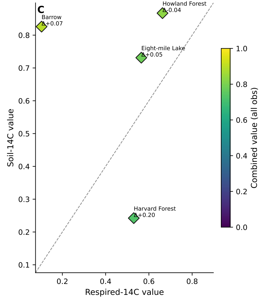
Value of Soil, Respired, and Combined Radiocarbon
