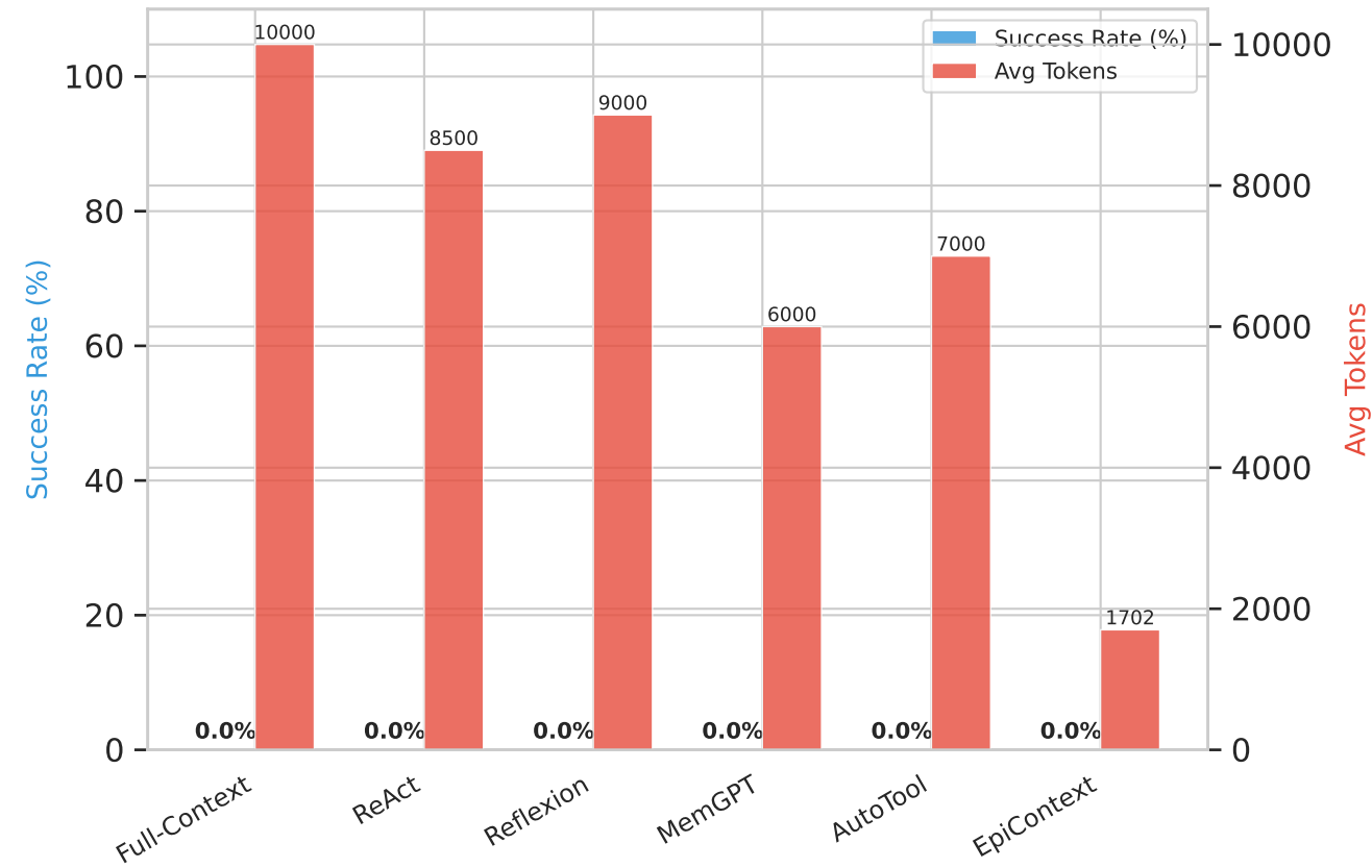
AGENTBENCH
