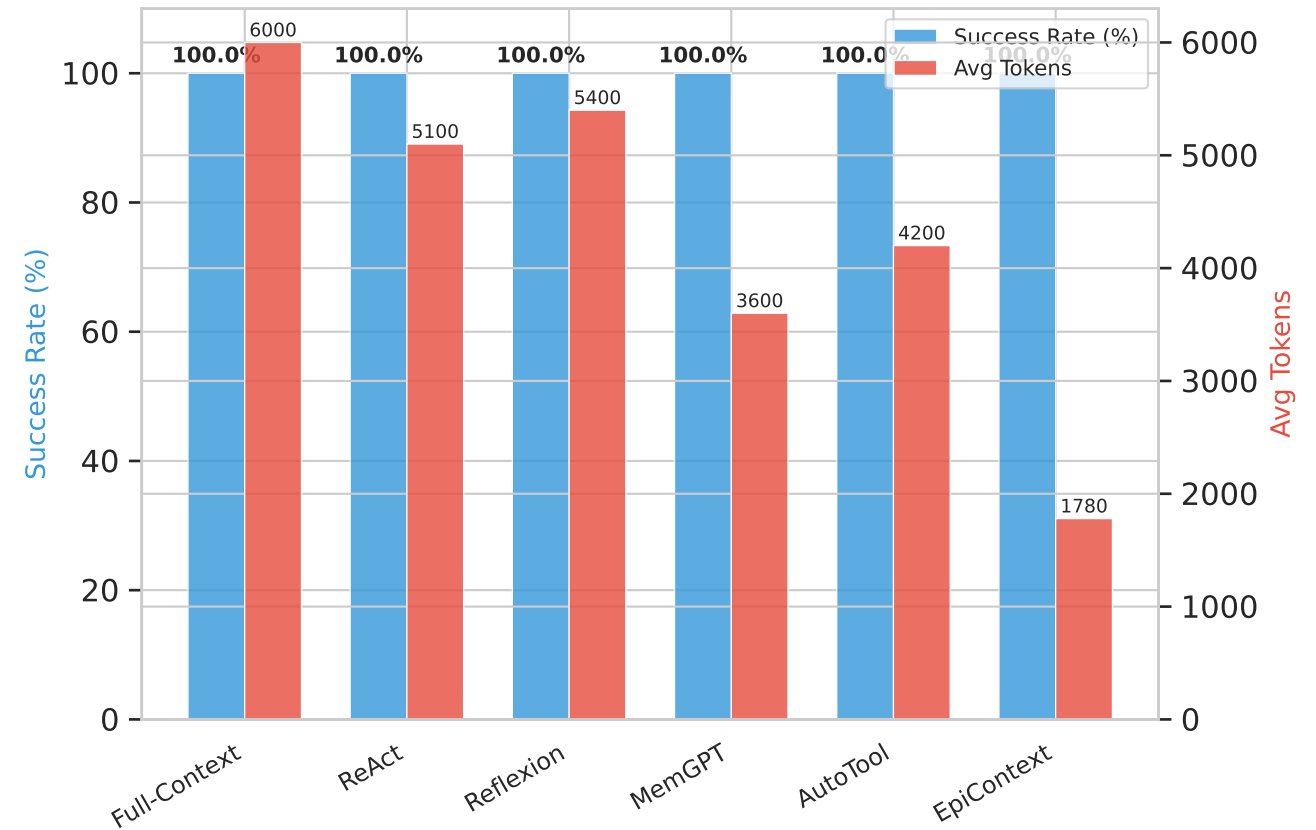
SWEBENCH
