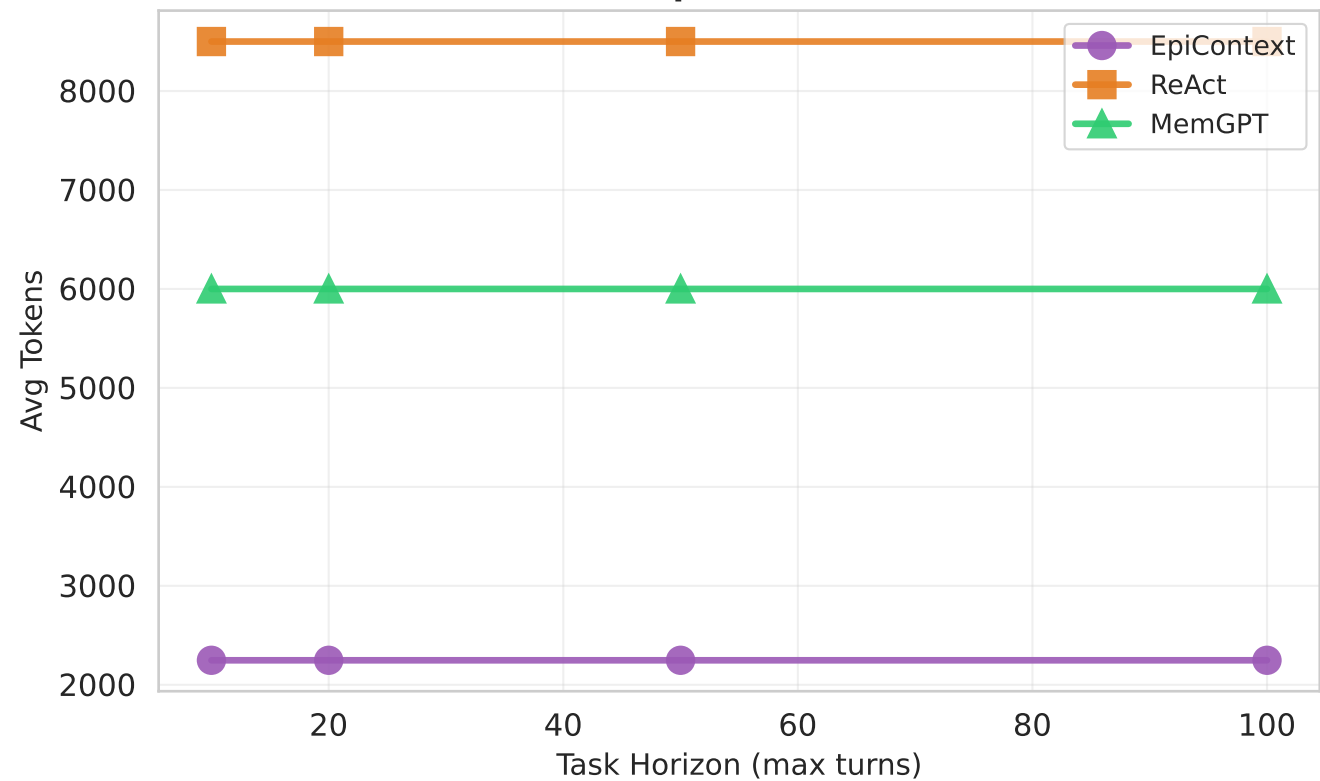
Token Consumption vs Task Horizon
