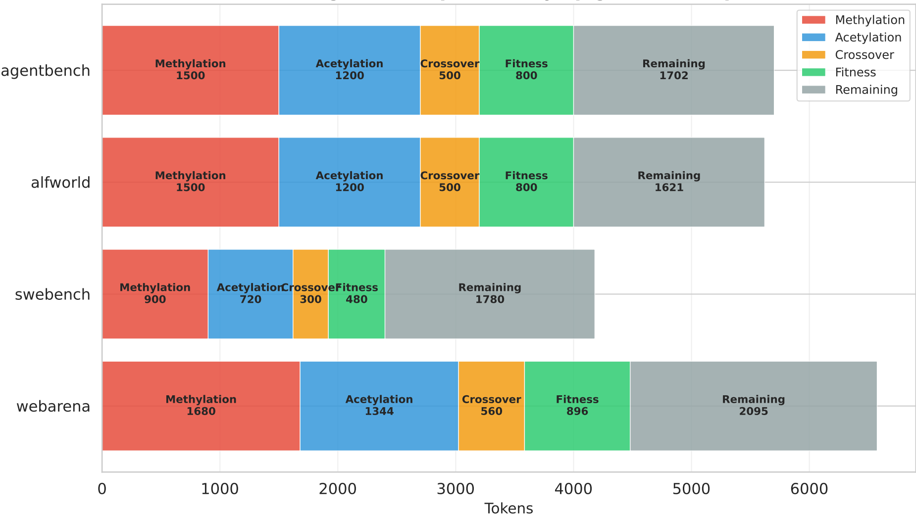
Token Budget Decomposition by Epigenetic Component
