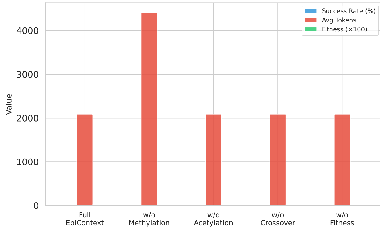
Ablation on WEBARENA
