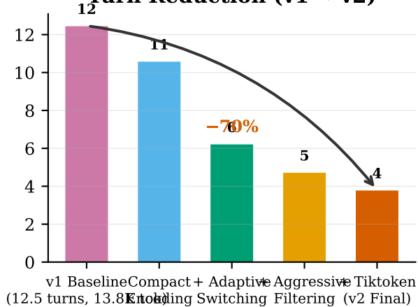
Turn Reduction (v1 → v2)
