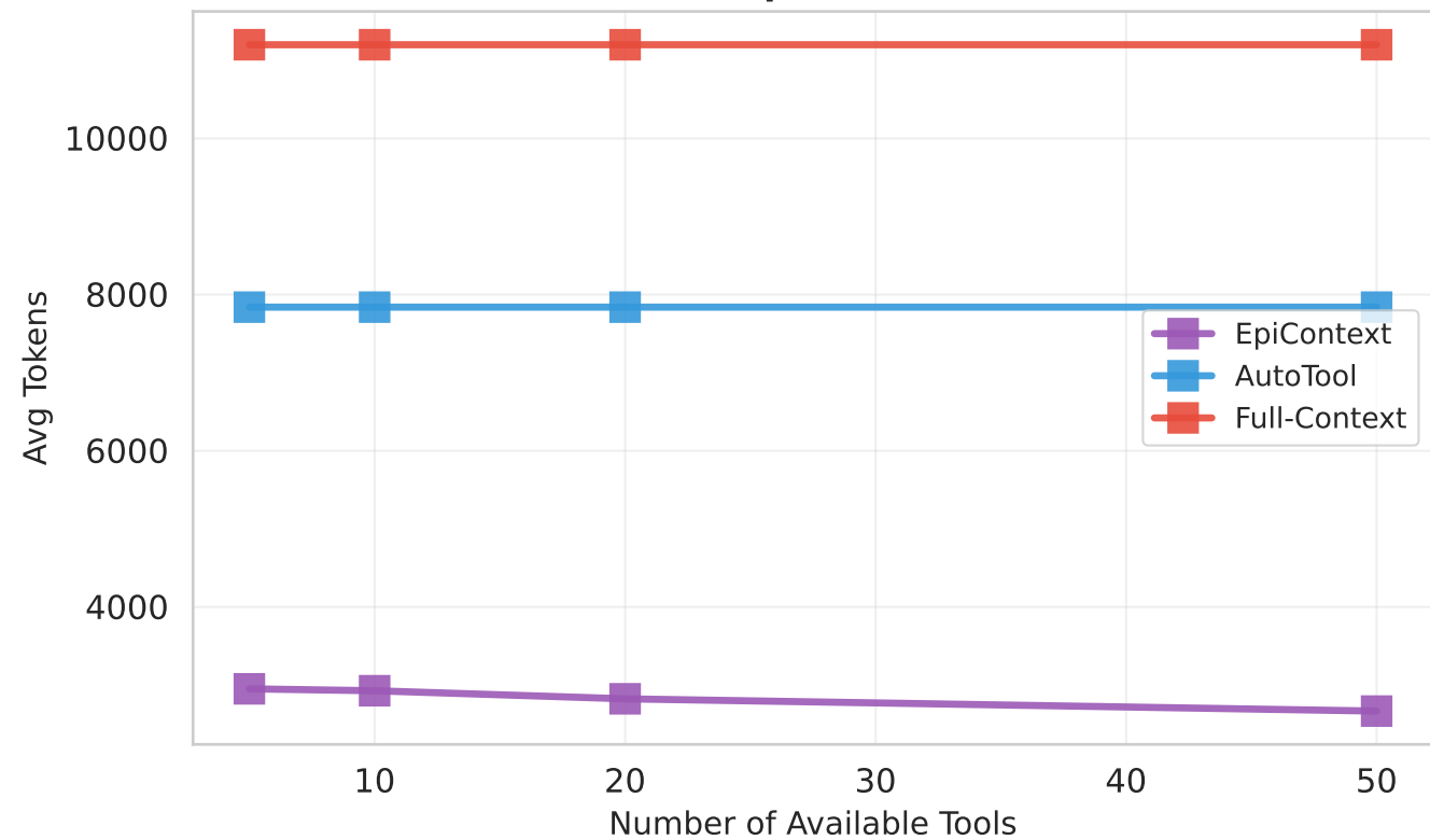
Token Consumption vs Tool Count
