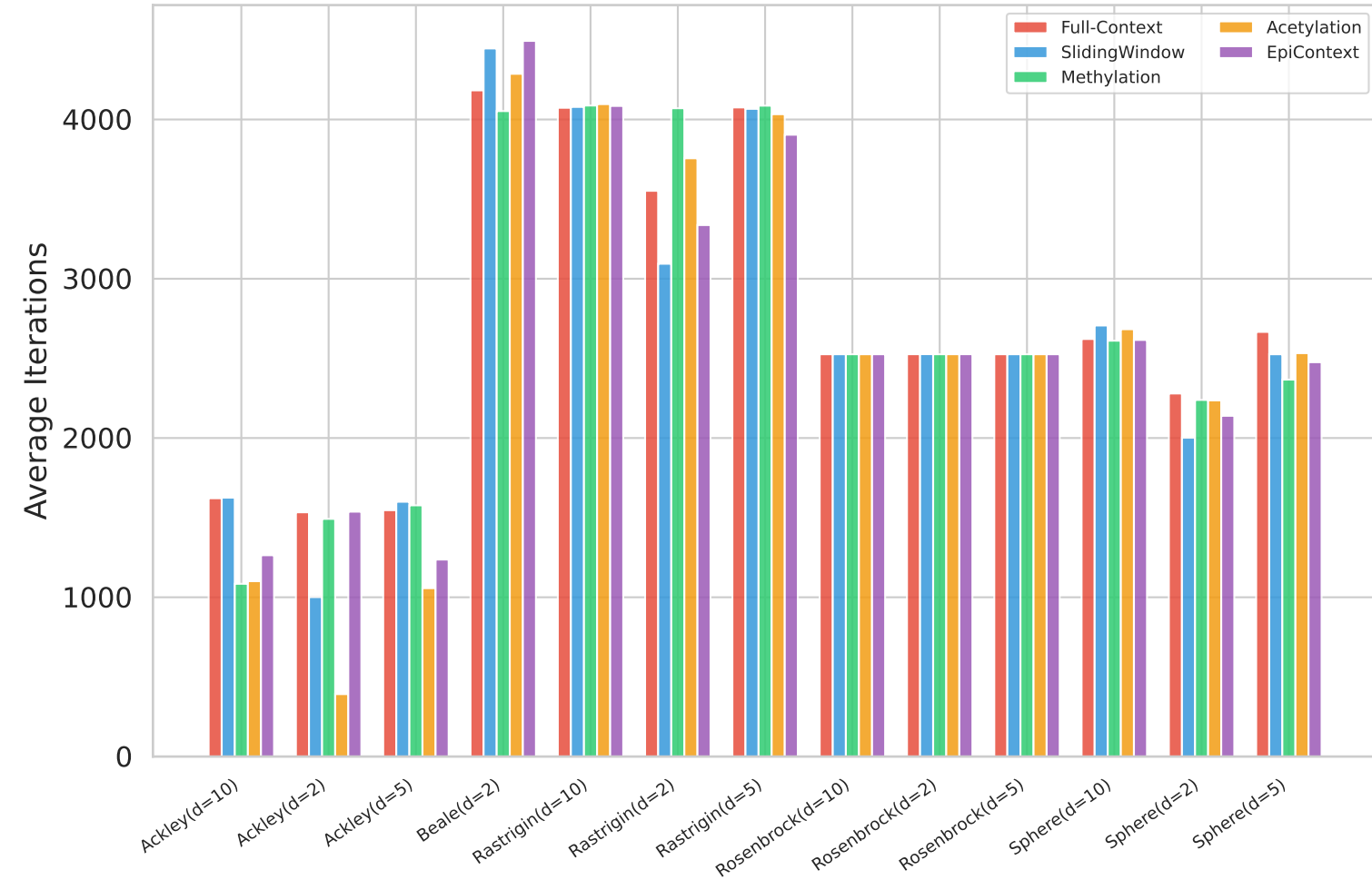
Iterations to Convergence
