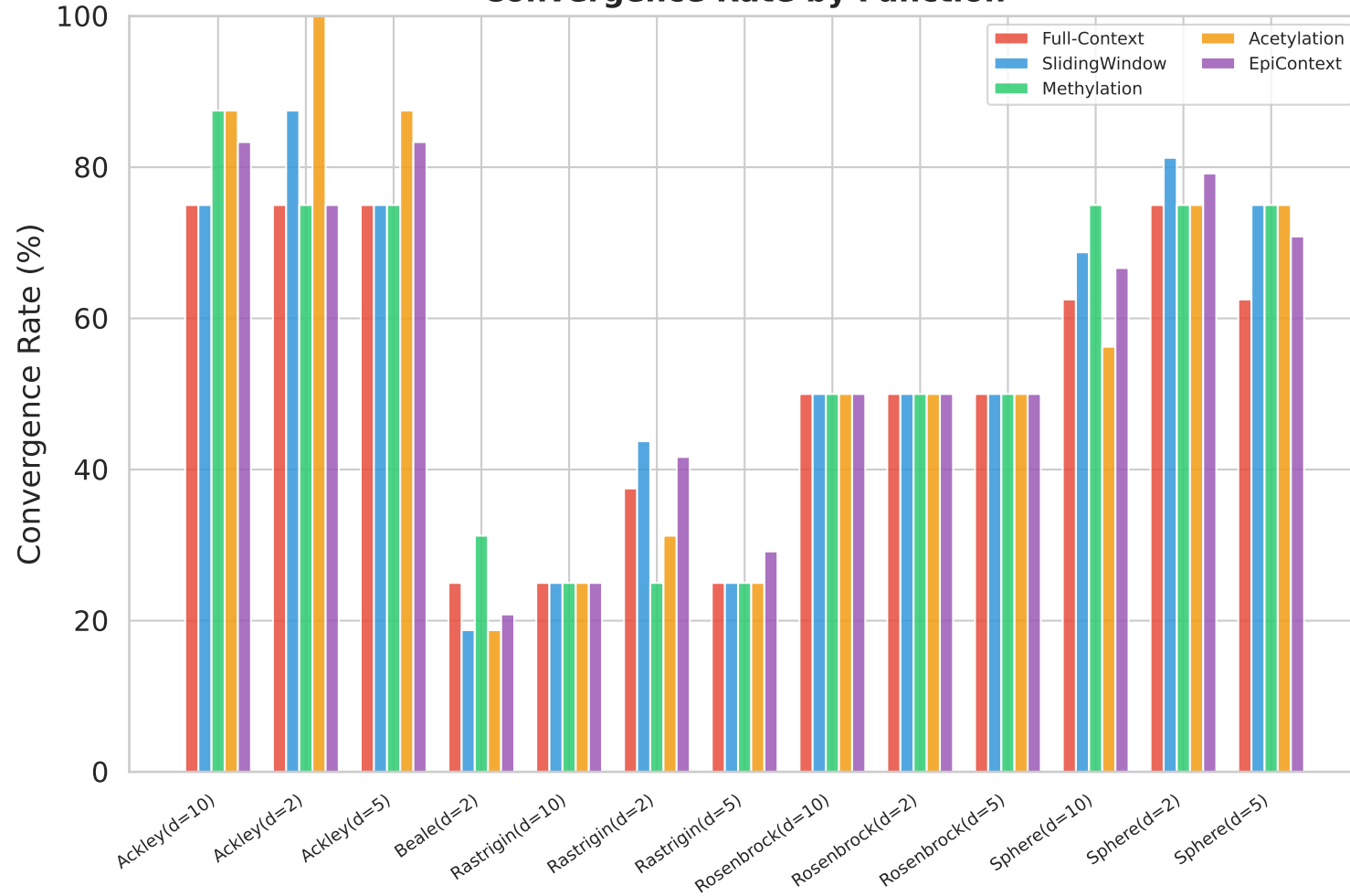
Convergence Rate by Function
