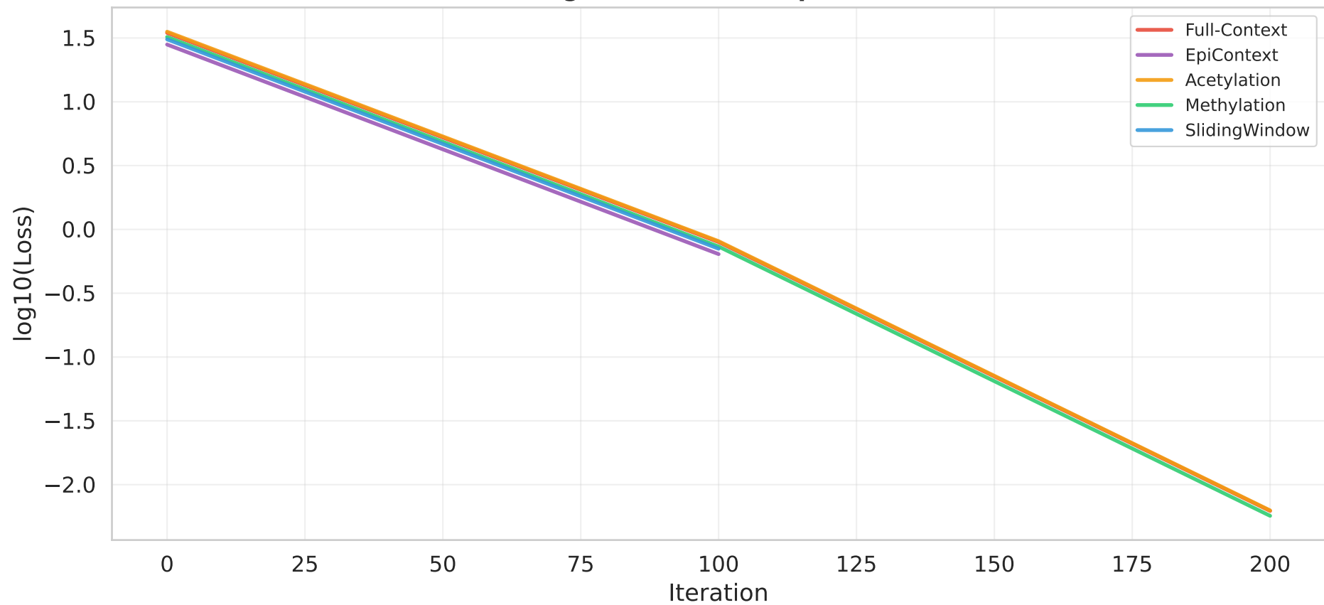
Average Loss Curves: Sphere(d=5)
