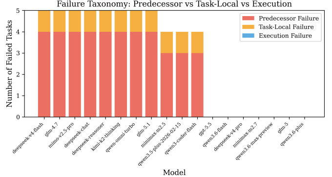
Fig. 4: Failure taxonomy composition. Predecessor failure dominates without resurrection but is largely eliminated by resurrection, revealing the underlying task-local and execution failure distribution.
