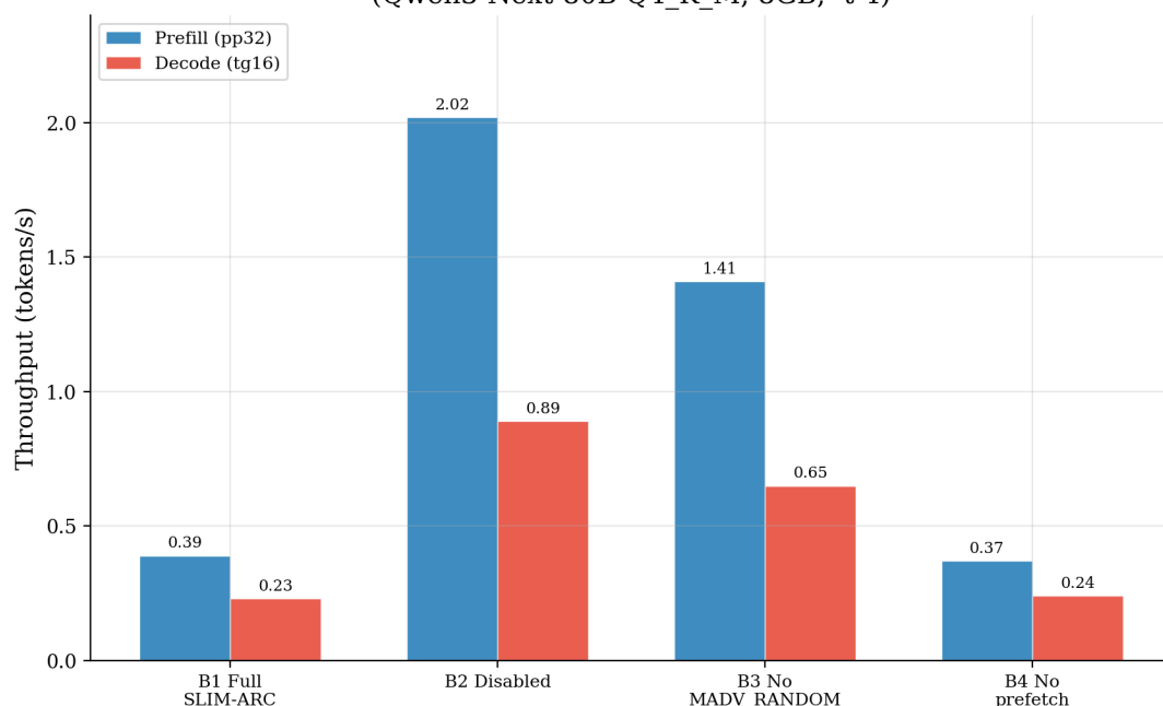
RK3588: switch ablation - MADV_RANDOM is the main overhead (Qwen3-Next-80B Q4_K_M, 8GB, -t 4)
