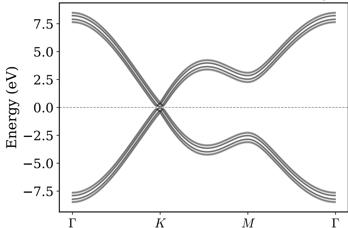
TB band structures at selected E_z
