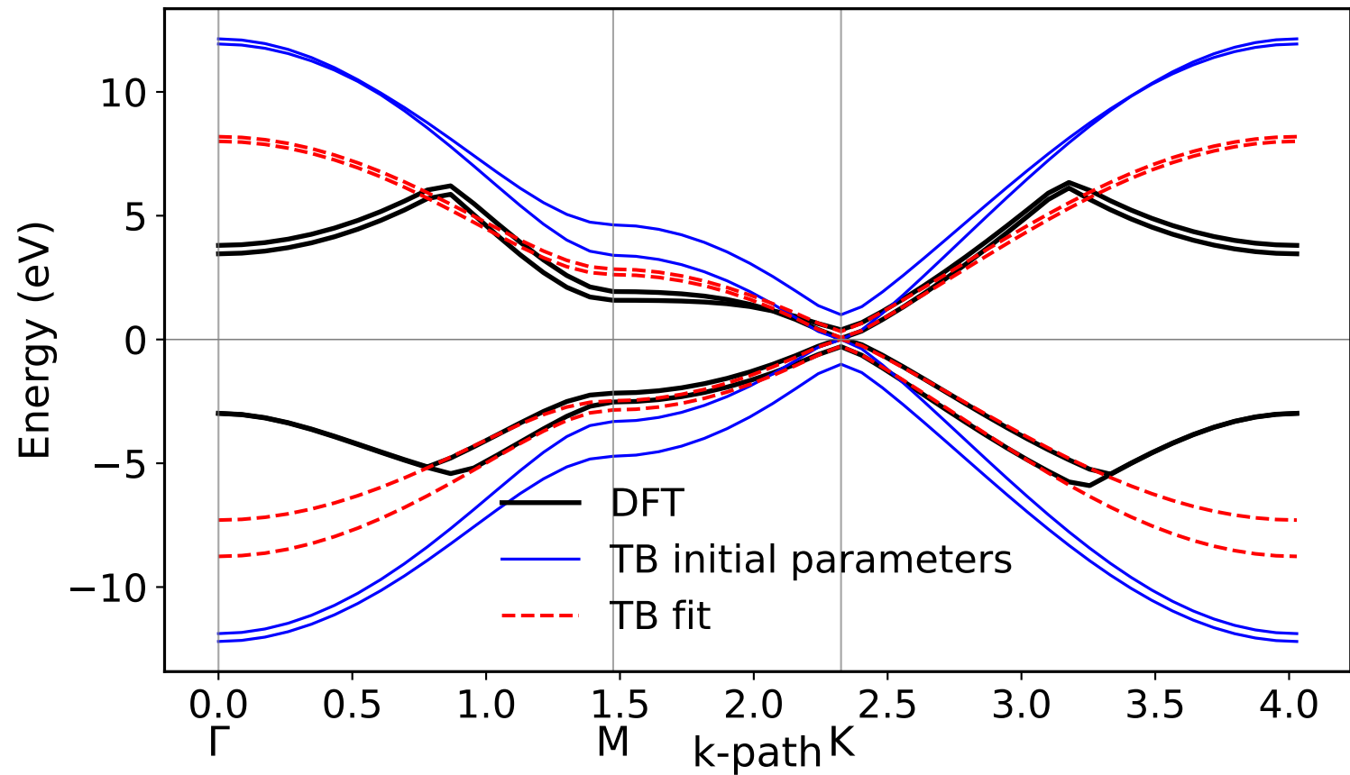
DFT vs TB bands
