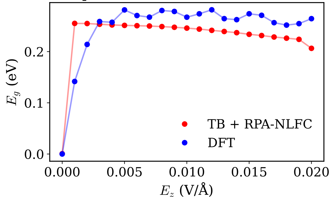
Gap vs External Field (RPA-NLFC)
