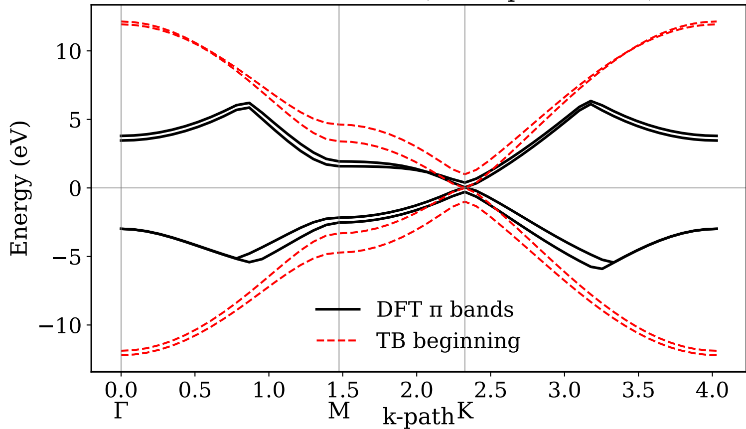
DFT \pi Bands vs TB (initial parameters)
