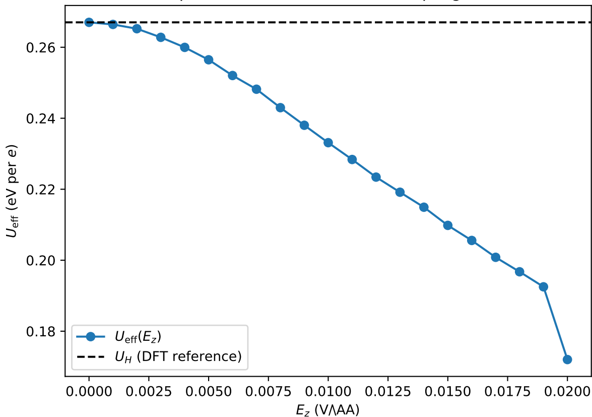
Field-dependent effective Hartree coupling from RPA
