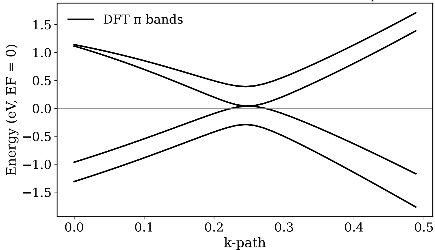
DFT \pi Bands zoomed on K — Parabolic Dispersion
