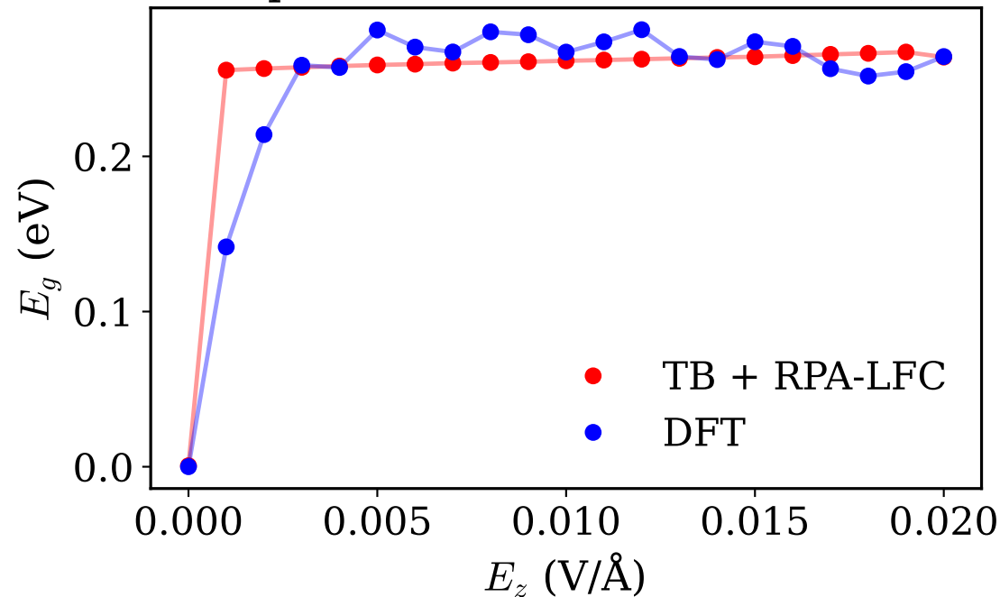
Gap vs External Field (RPA-LFC)
