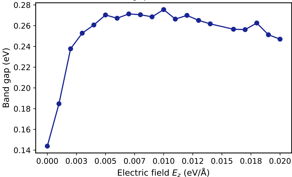
Band gap vs electric field
