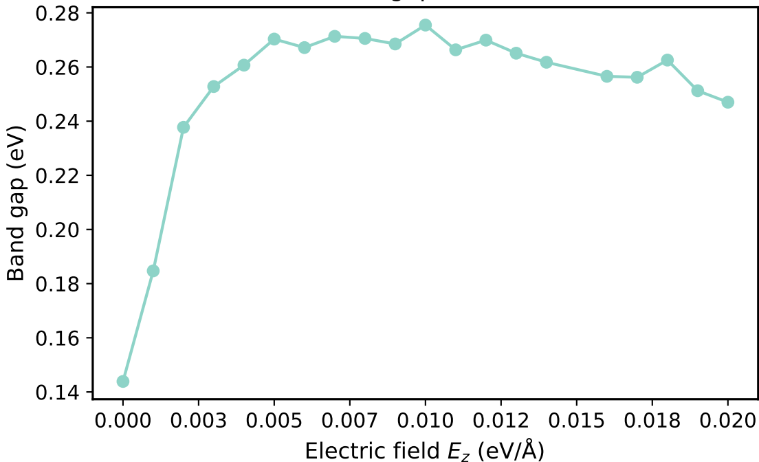
K-zoom band gap vs electric field
