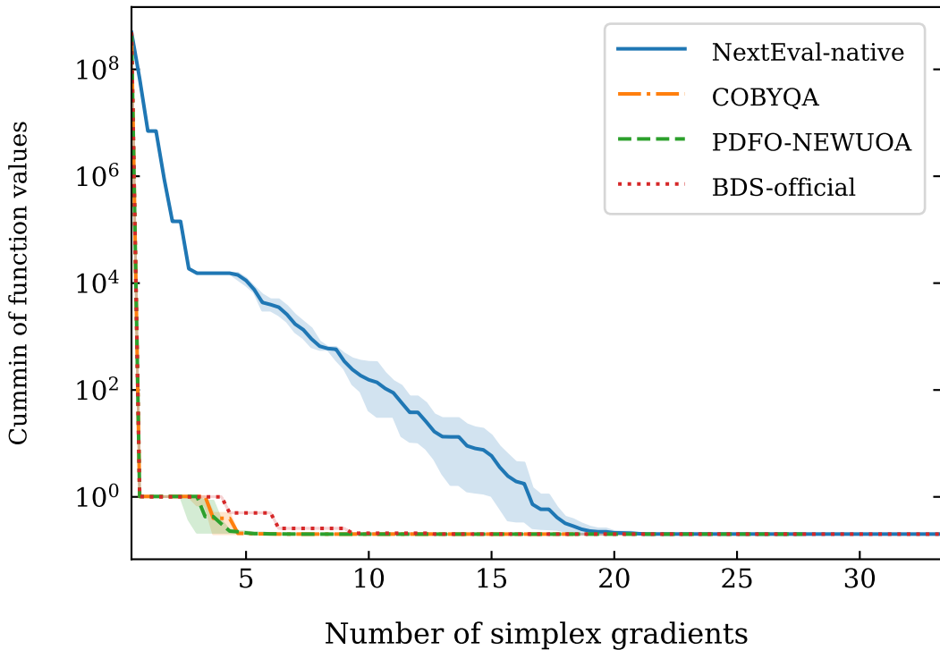
Solving "CLIFF" with "perturbed_x0_noisy" feature
