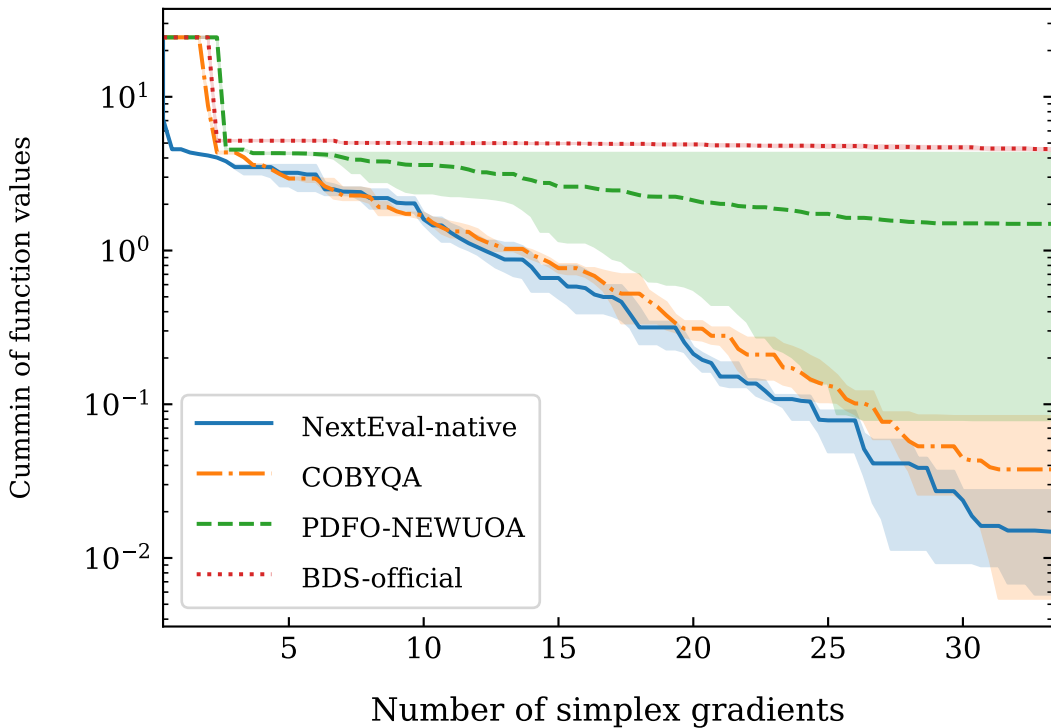
Solving "ROSENBR" with "perturbed_x0_noisy" feature
