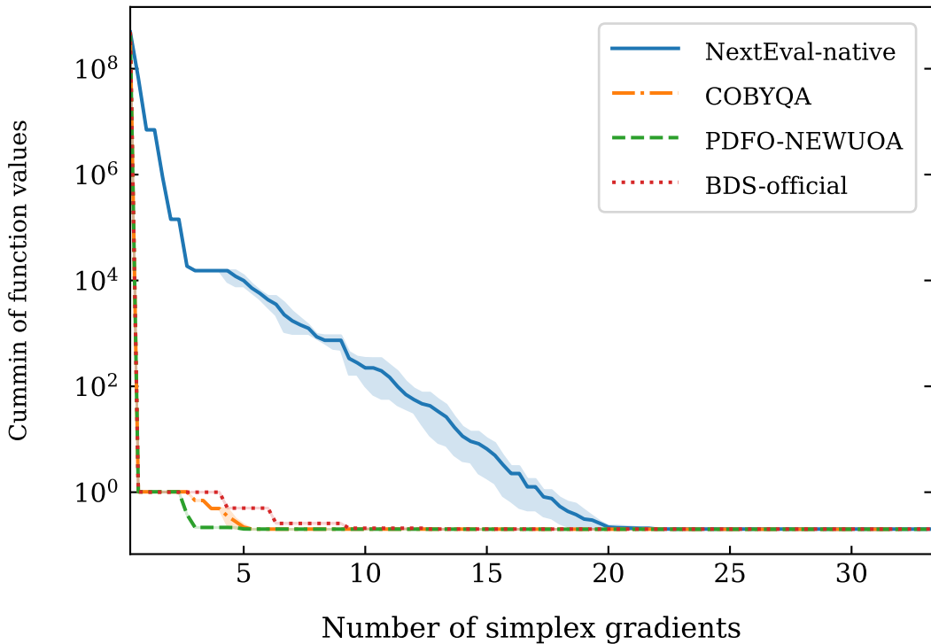
Solving "CLIFF" with "perturbed_x0" feature
