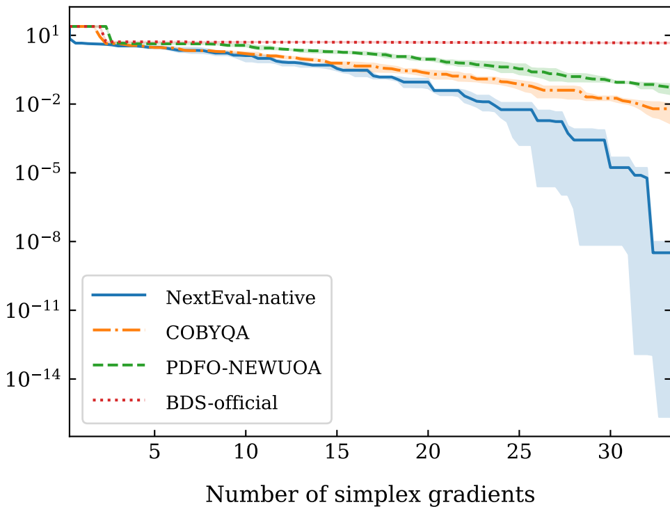
Solving "ROSENBR" with "perturbed_x0" feature
