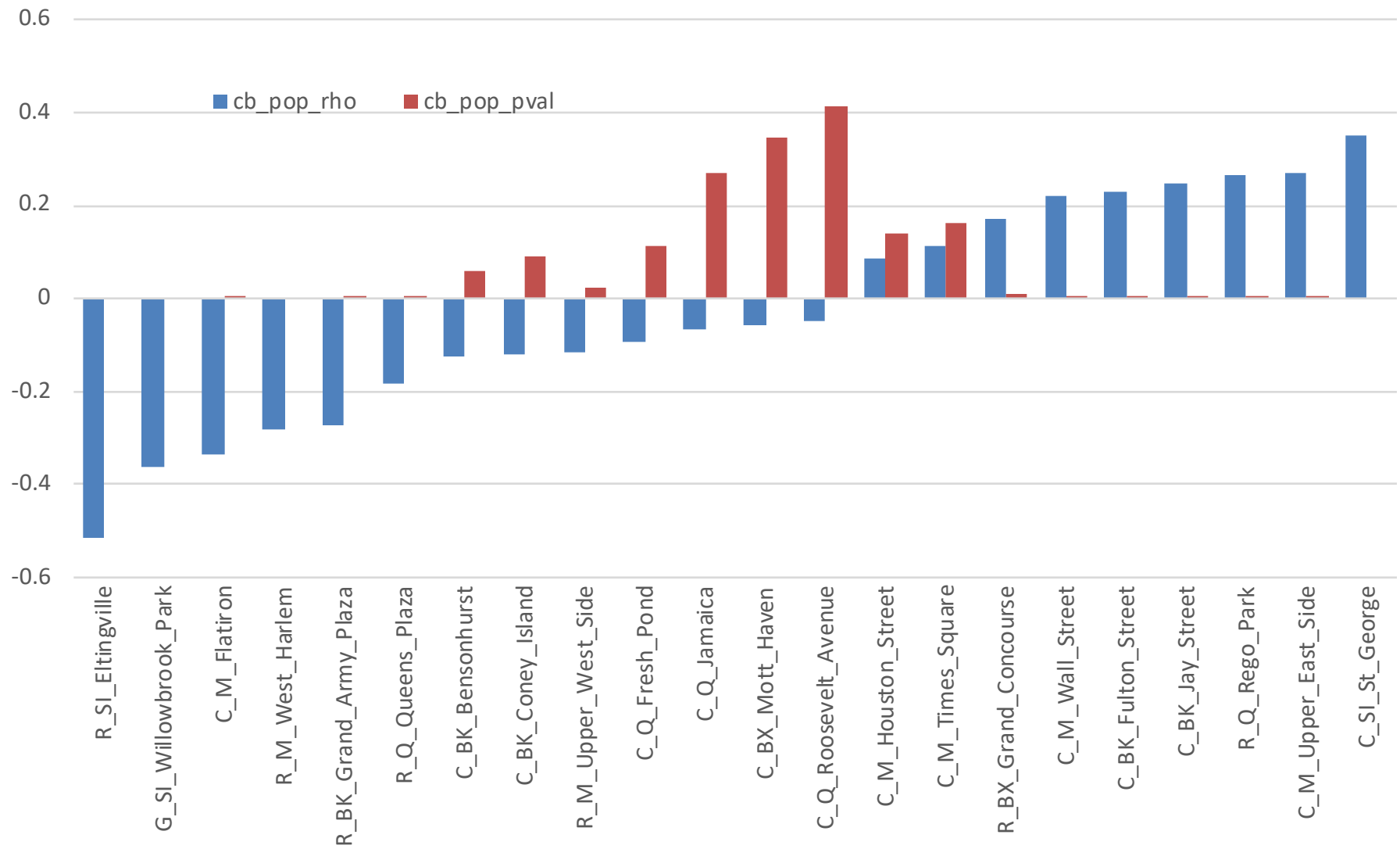
Spearman Rank Correlation: Census Block Population vs Total RMS by Path
