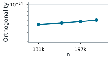
FP64
