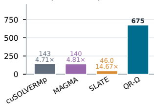
TF32, n = 131,072
