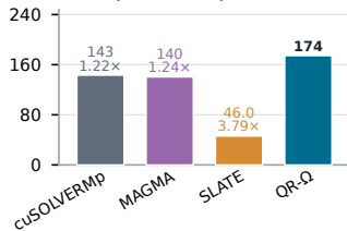
FP32, n = 131,072
