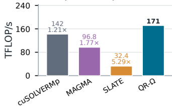
FP64, n = 131,072
