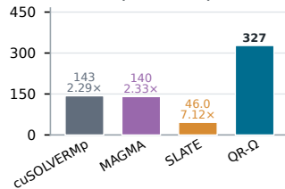
3×TF32, n = 131,072
