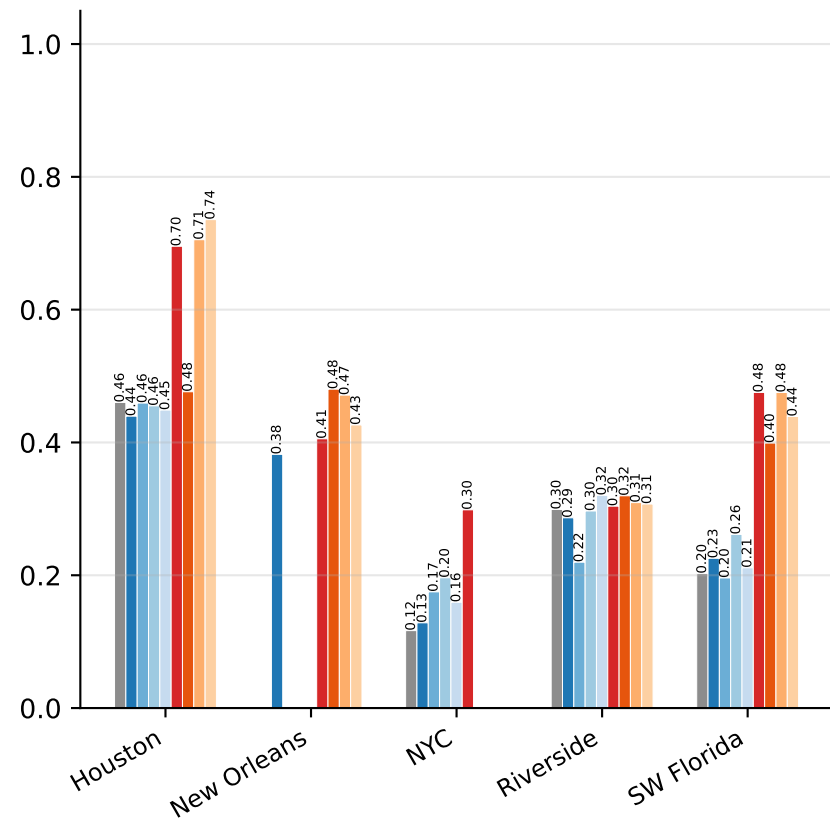
NFIP Claims ( R^2 )
