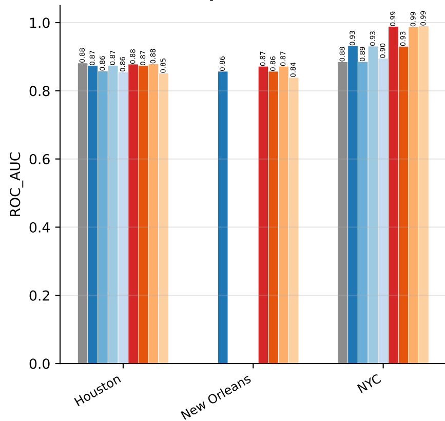
311 Reports (ROC-AUC)
