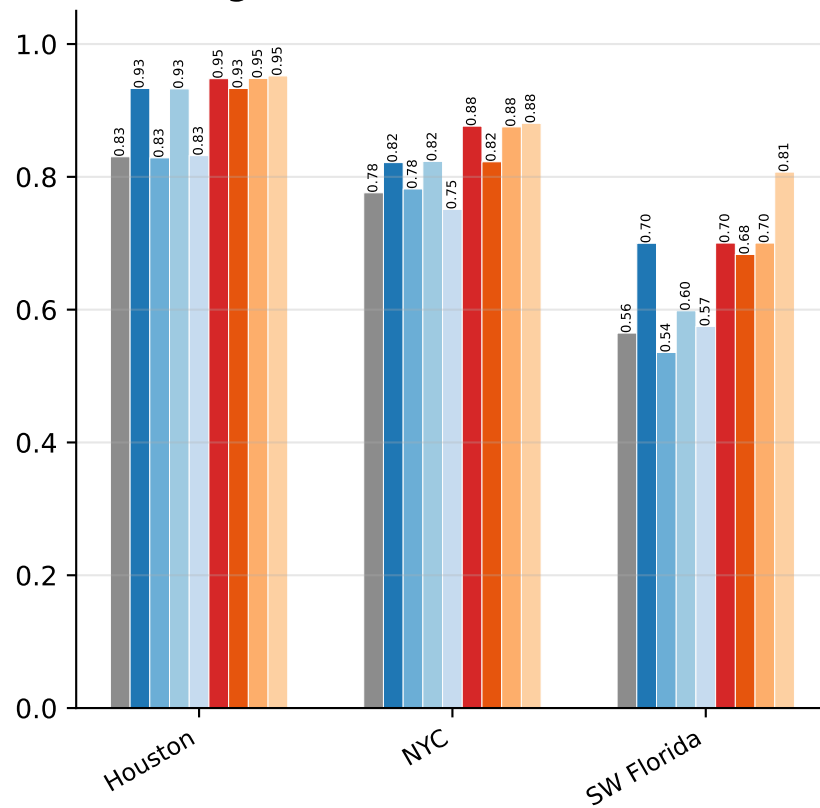
High Water Marks (ROC-AUC)
