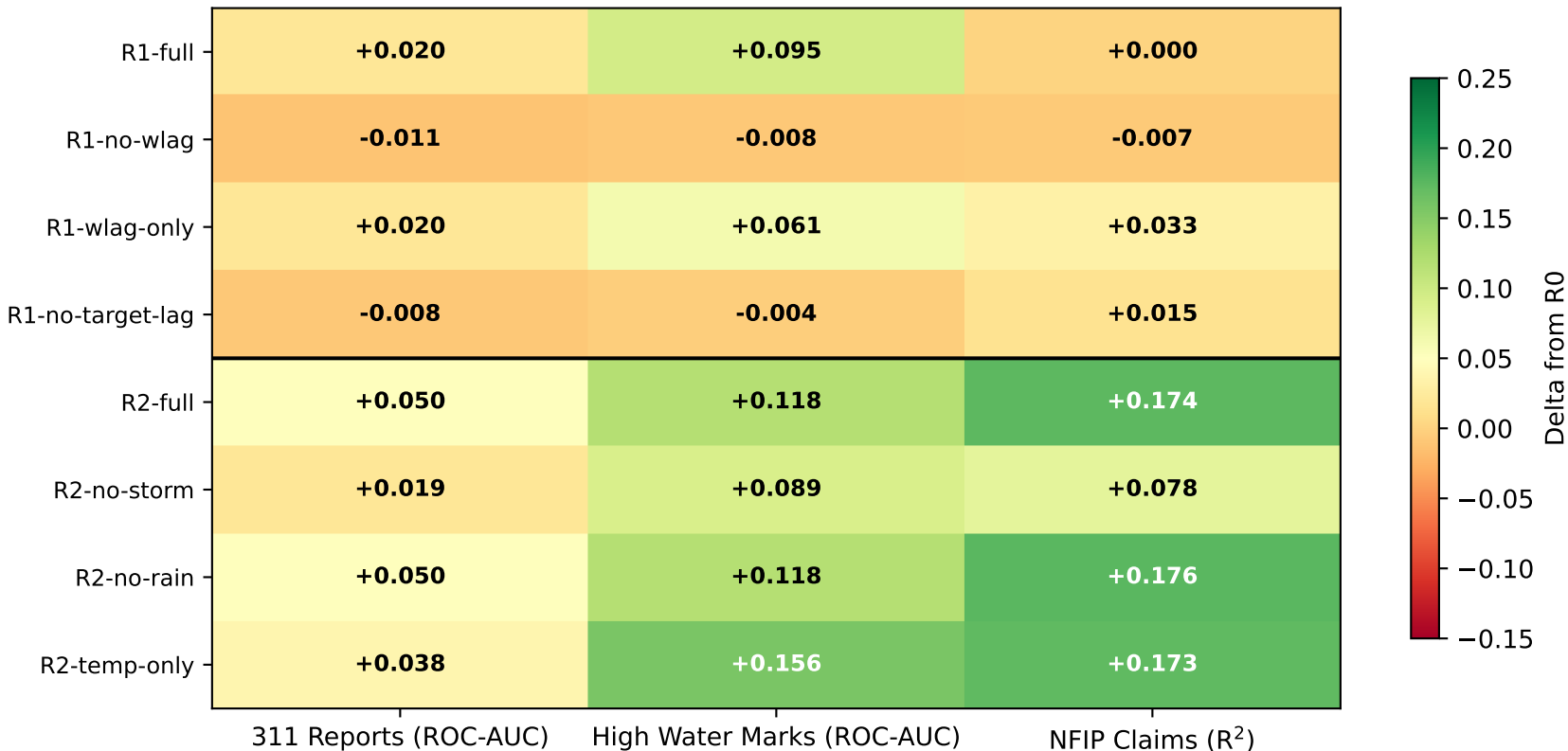
Feature Sub-Group Contribution (delta from R0 baseline)
