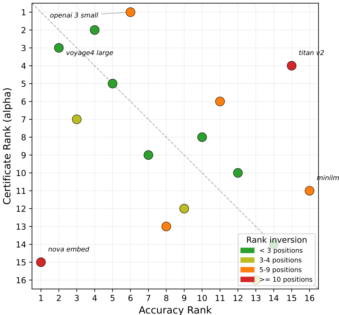
The Certification Gap: Accuracy vs Certificate Rank Spearman \rho = 0.31 | 9/16 models inverted \geq 3 positions
