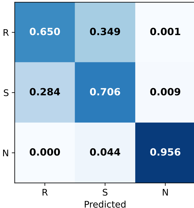
nova_embed Accuracy #1 (77.1%) | Alpha #15 (0.483)
