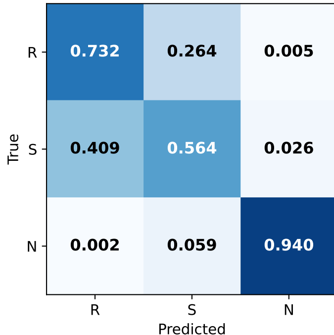
openai_3_small Accuracy #6 (74.5%) | Alpha #1 (0.514)
