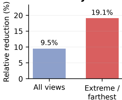
W-MPJPE
