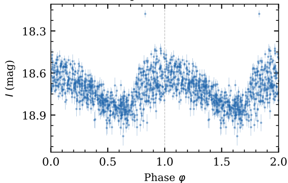
RR Lyrae d — first overtone P_2 = 0.49098 \sim d
