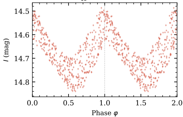
Cepheid F/1O — 1O mode P_{1O} = 3.63156 \sim d
