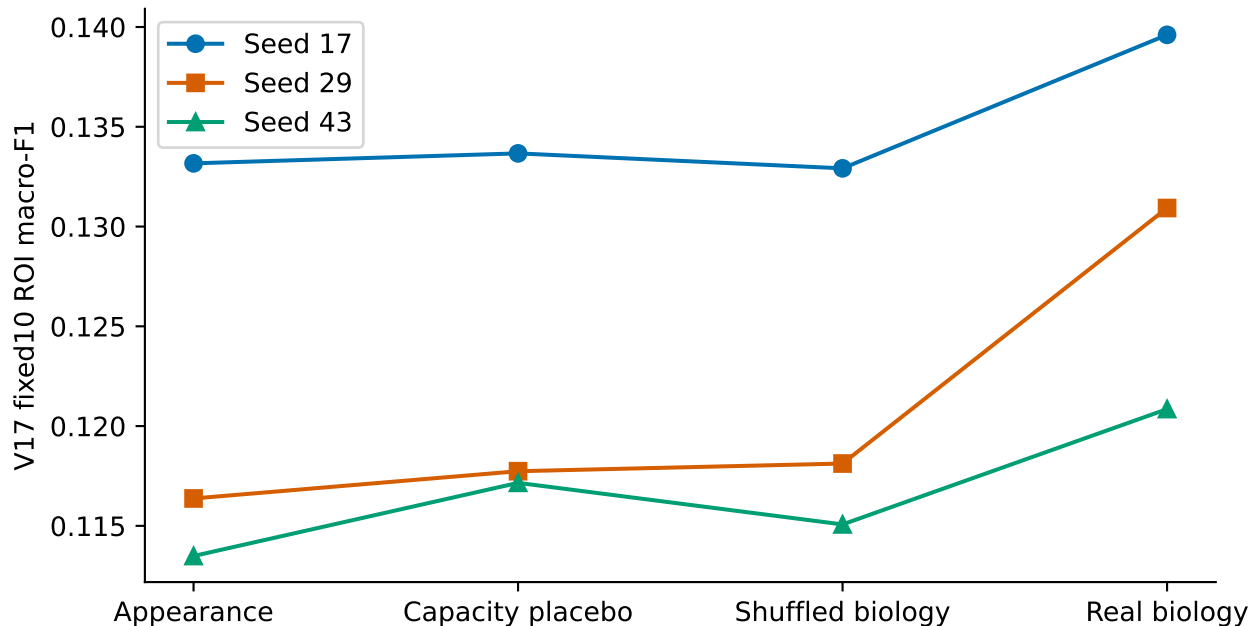
Matched seed controls (150 validation features / 40 ROIs)
