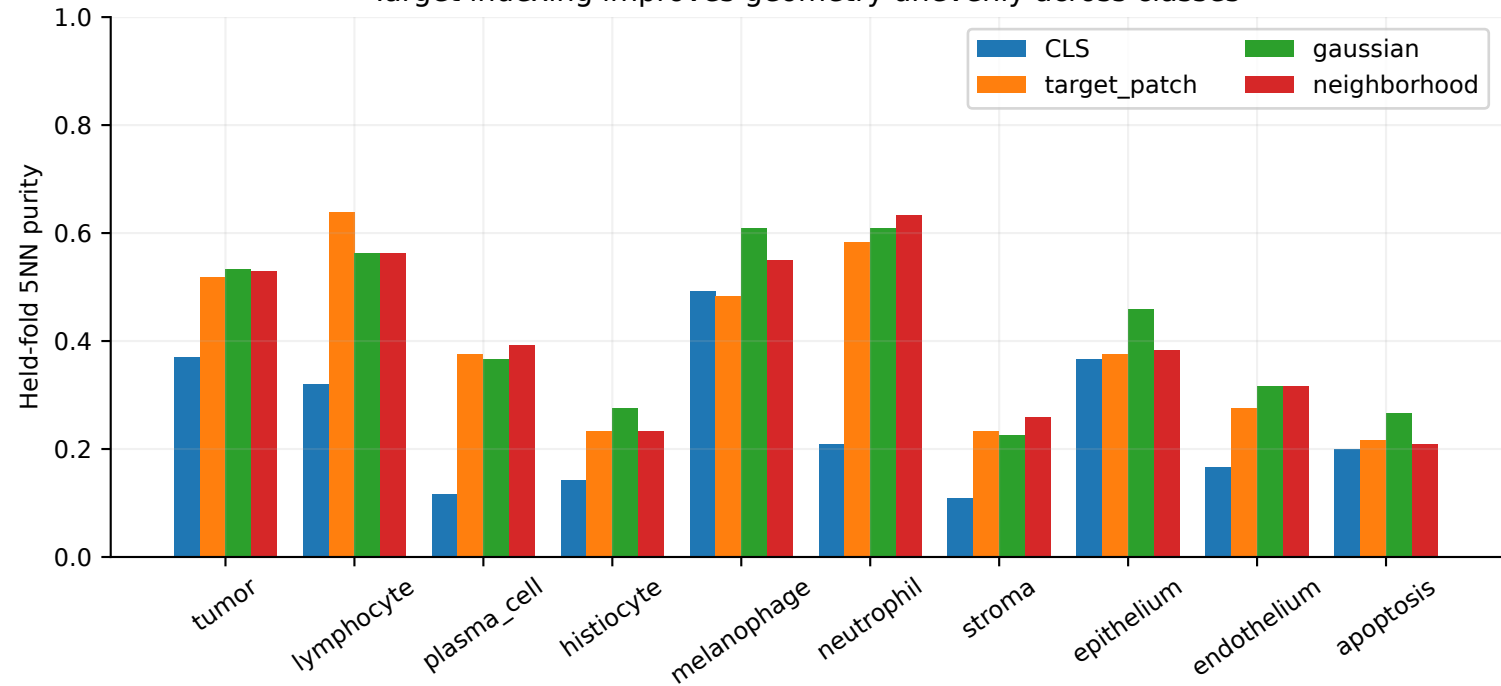
Target indexing improves geometry unevenly across classes
