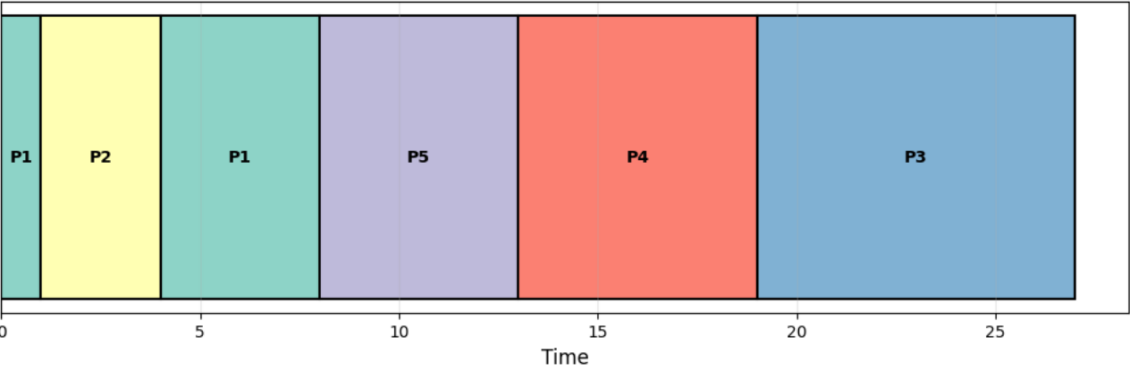
Gantt Chart
