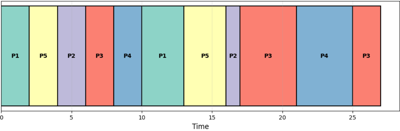
Gantt Chart
