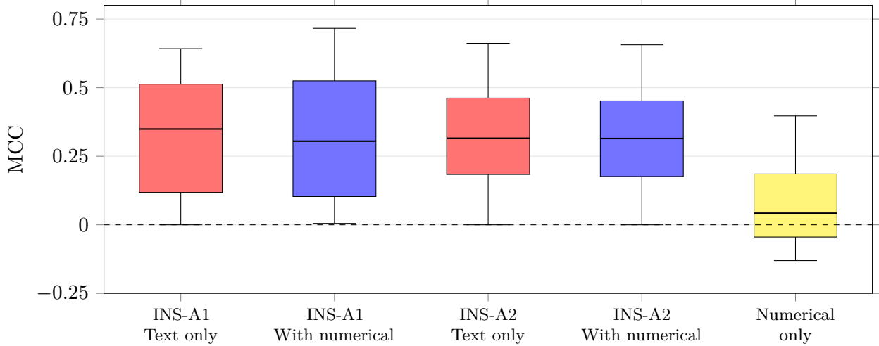
Figure 2: Insufficiency: distribution of MCC across 25 depth- \leq 2 case-grouped validation splits. Boxes show the interquartile range, horizontal lines show medians, and whiskers show the observed minimum and maximum.
