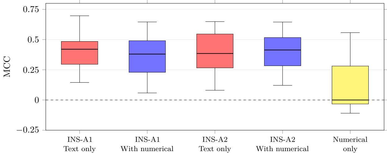
Figure 3: Insufficiency: distribution of MCC across 25 full-depth ( \leq 100 ) case-grouped validation splits. Boxes show the interquartile range, horizontal lines show medians, and whiskers show the observed minimum and maximum.
