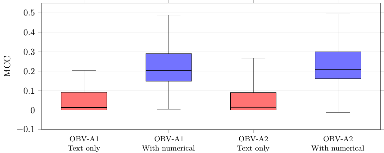
Figure 4: Obviousness: distribution of MCC across 50 depth- \leq 2 case-grouped validation splits. Boxes show the interquartile range, horizontal lines show medians, and whiskers show the observed minimum and maximum.
