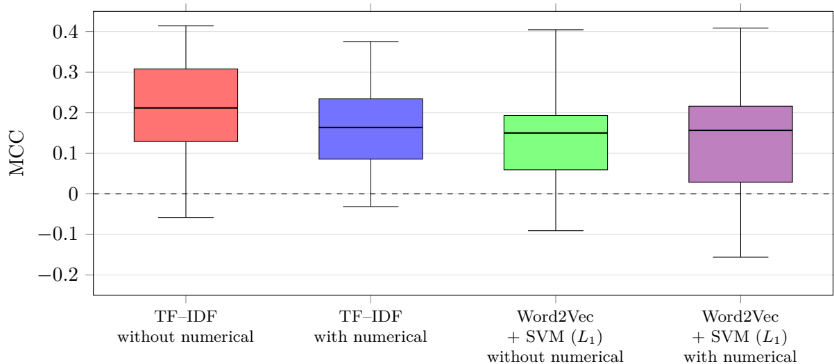
Figure 1: Distribution of MCC across 50 case-grouped validation splits. Boxes show the interquartile range, horizontal lines show medians, and whiskers show the observed minimum and maximum.
